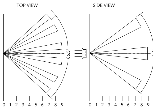
85° x 75° Distribution
