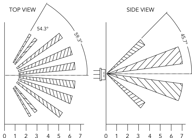
120° x 90° Distribution
