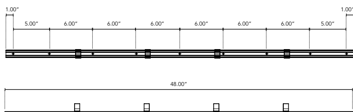
Plan View
