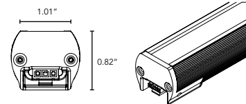
End View
