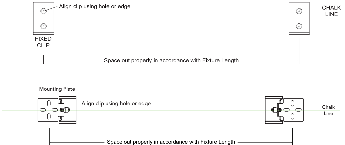
FIGURE A: CLIP ALIGNMENT
