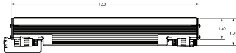
2 ELEVATION VIEW
