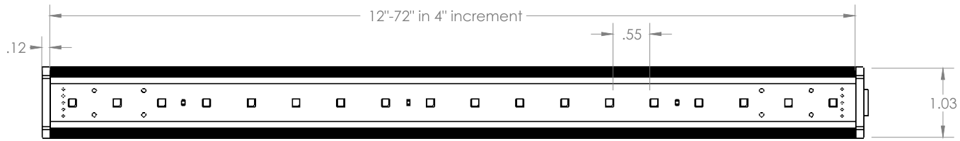
1 PLAN VIEW
