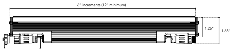
Elevation View
