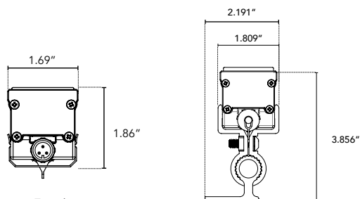
Fixed
