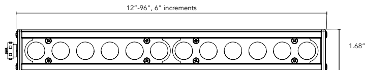
Plan View
