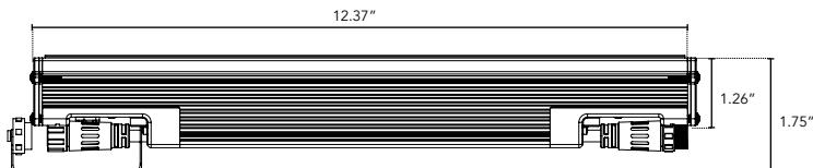
Elevation View
