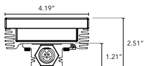
End View
