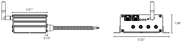
Elevation View
