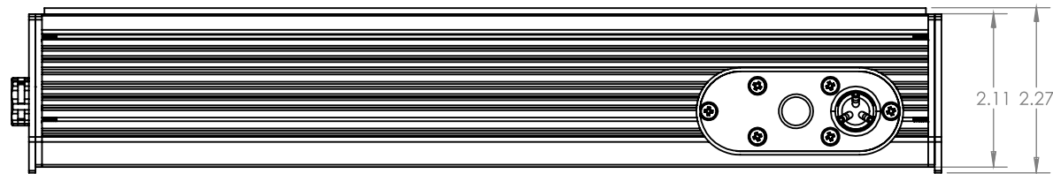
2 ELEVATION VIEW
